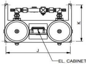
EL. CABINET
